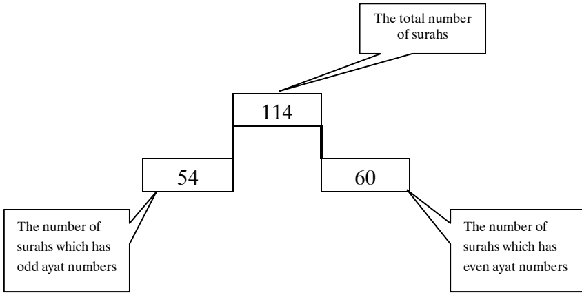
Figure-1 The distribution of the surahs with respect to ayat numbers is seen.
