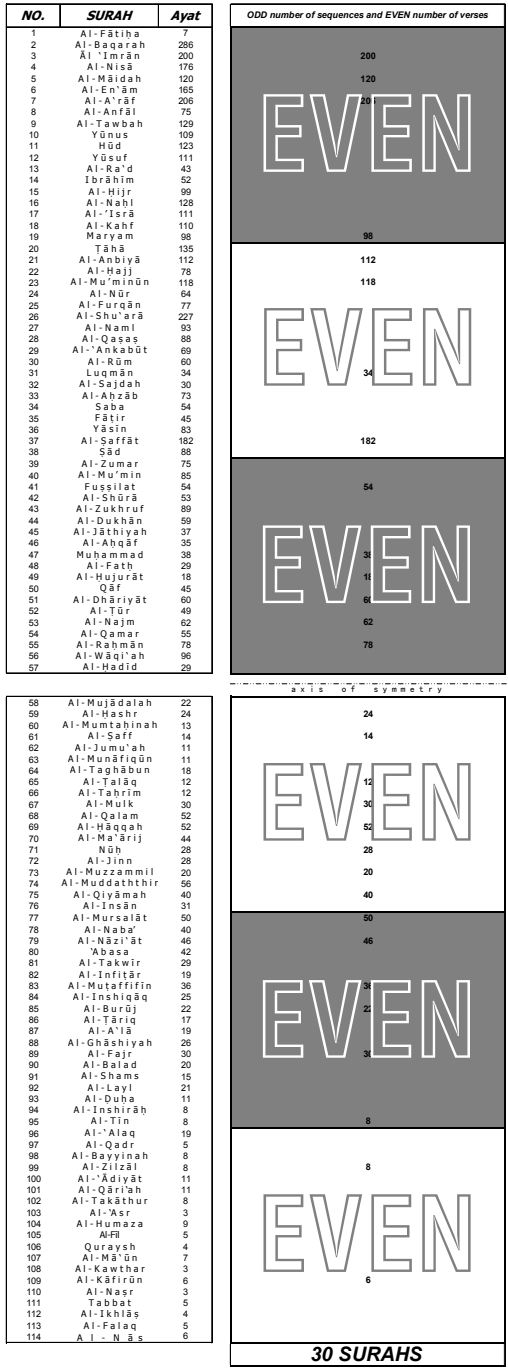
Symmetric distribution of the number of verses for surahs with odd number of sequences and even number of verses in groups of 19 is shown in the Figure.
