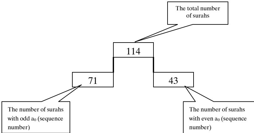
Figure-21 Distribution of the surahs (as prime and prime) is shown.
