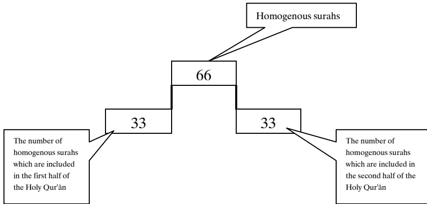
Figure-10 The equal distribution of the homogeneous surahs is seen.
