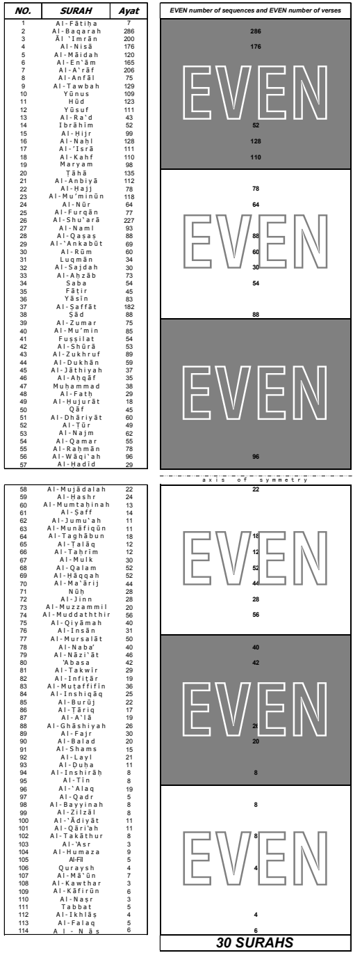
Symmetric distribution of the number of verses for surahs with even number of sequences and even number of verses in groups of 19 is shown in the Figure.
