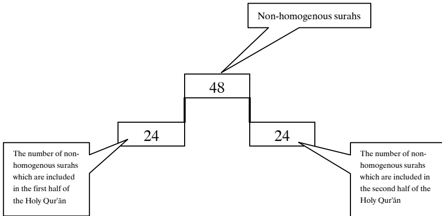
Figure-11 The equal distribution of the non-homogenous surahs is seen.
