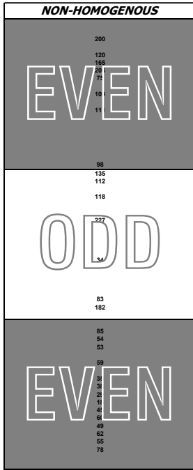
Symmetric distribution of the number of verses for the non-homogenous surahs in groups of 19 is shown in the Figure.
