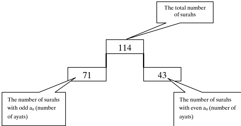
Figure-20 Distribution of the surahs (as prime and prime) is shown.
