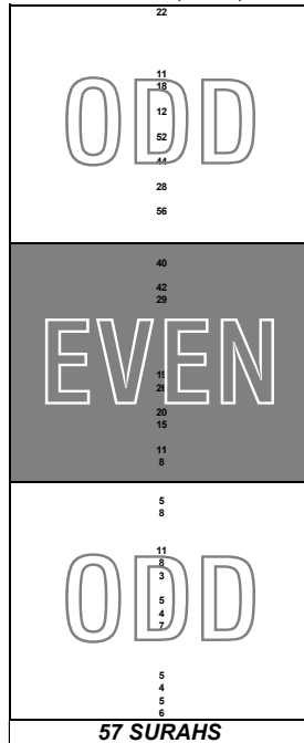
Symmetric distribution of the number of verses for the homogenous surahs in groups of 19 is shown in the figure.
