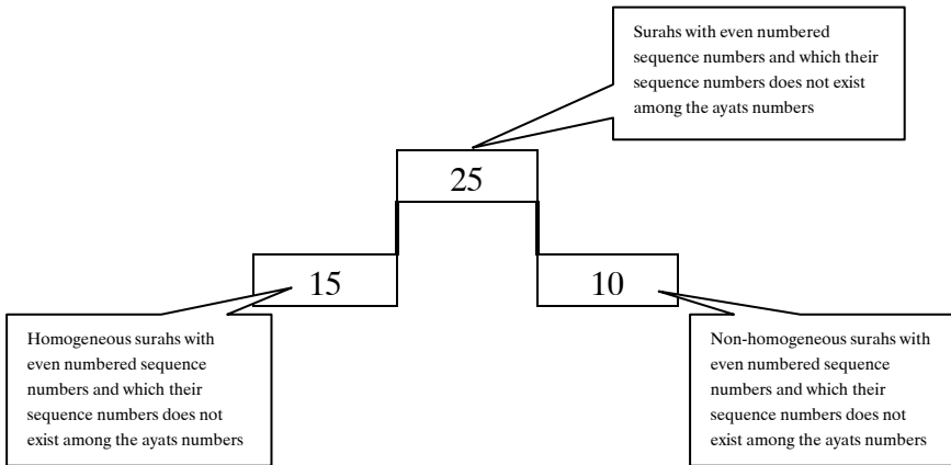
Figure-9 Distribution of the surahs with even numbered sequence numbers and which their sequence numbers does not exist among the ayats numbers is seen.
