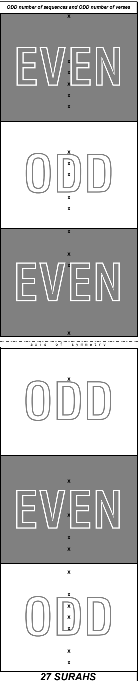
Symmetric distribution of the surahs with odd number of sequences and odd number of verses in groups of 19 is shown in the Figure.
