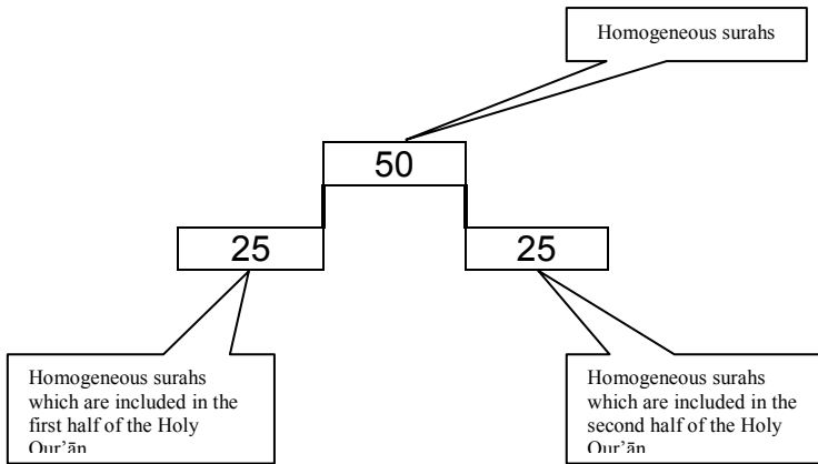
Figure-11 The equal distribution of the homogeneous surahs.
