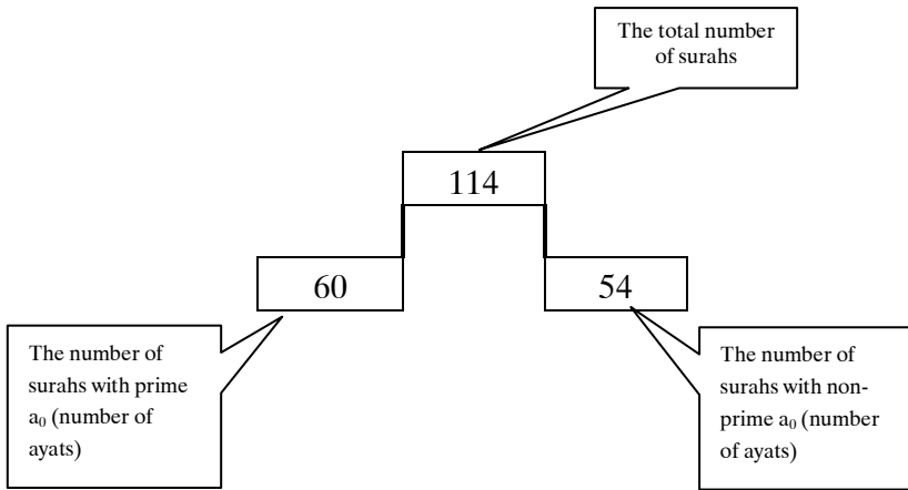
Figure-22 The distribution of the surahs with prime and non-prime number in a_0 (number of ayats) is seen.
