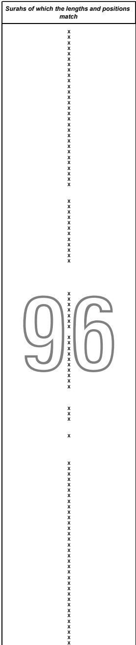
In the Figure, equal distributions of the surahs with matching situation and position of the number of verses with respect to the mean, and the surahs with matching lengths and positions are shown
