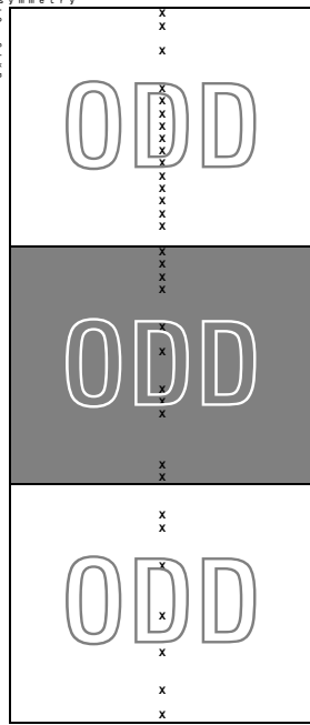
Symmetric distribution of the surahs with odd and even-number of verses in groups of 19 with respect to the number of surahs is shown in the Figure.
