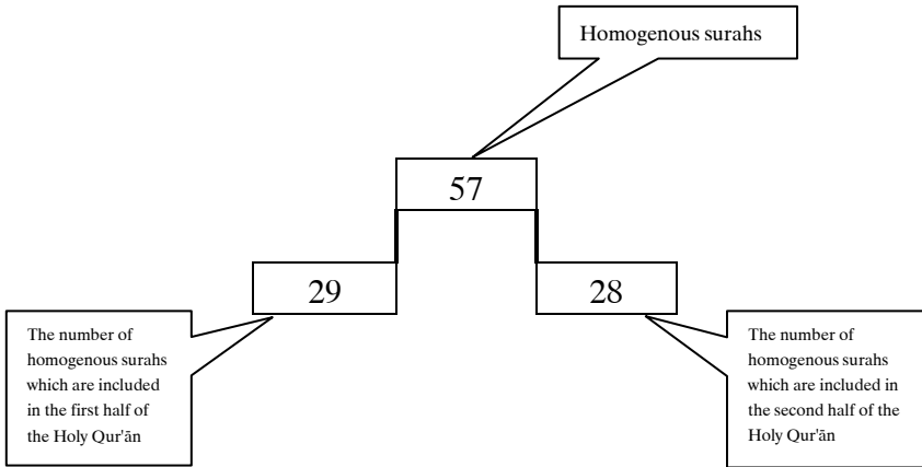
Figure-14 Distribution of the homogeneous surahs (as prime and non-prime) is shown.
