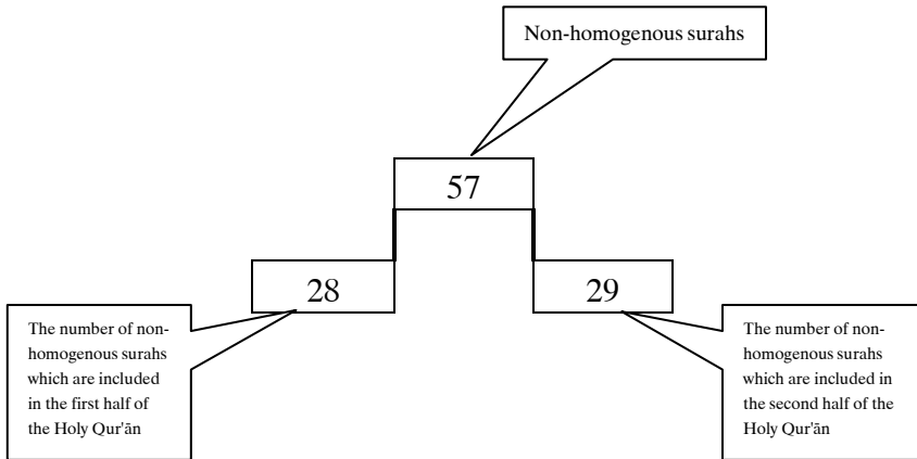
Figure-15 Distribution of the non-homogenous surahs (as prime and non-prime) is shown.
