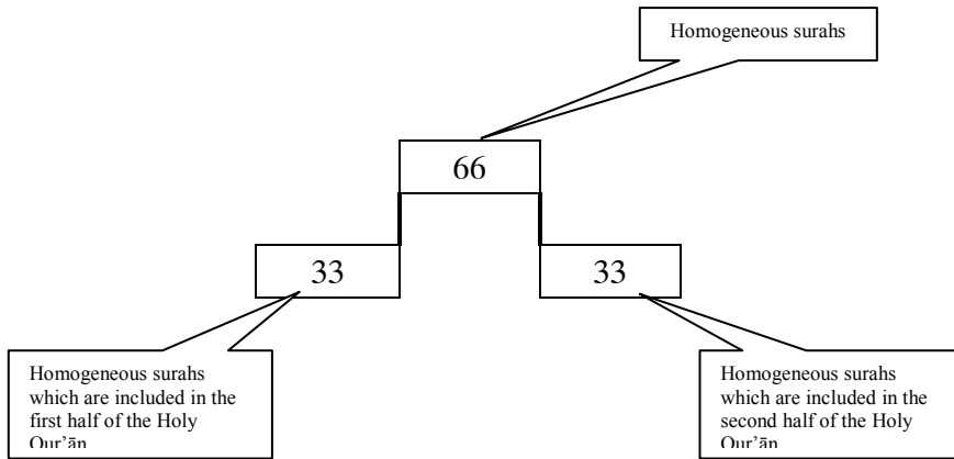
Figure-7 The equal distribution of the homogeneous surahs is seen.
