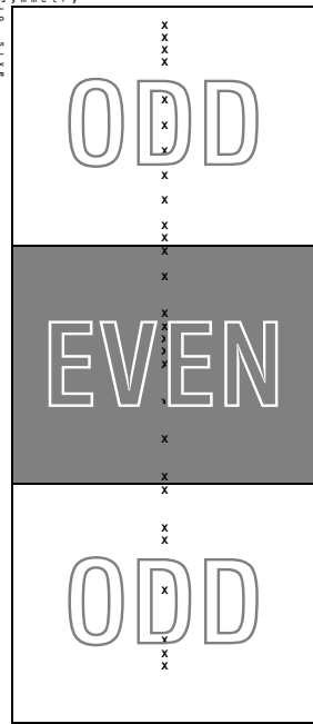
Symmetric distribution of the homogenous and non-homogenous surahs in groups of 19 is shown in the Figure.
