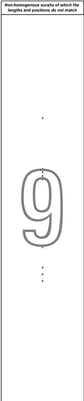
In the figure, equal distribution of the surahs of which the lengths and positions do not match is shown.
