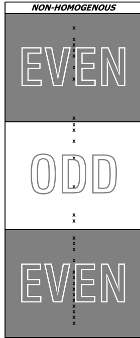
Symmetric distribution of the non-homogenous surahs in groups of 19 is shown in the Figure.
