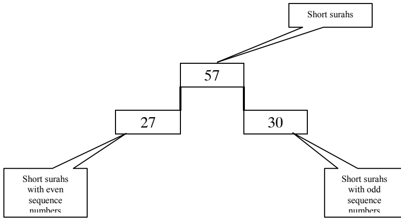
Figure-5 Distribution of the short surahs with respect to sequence number.
