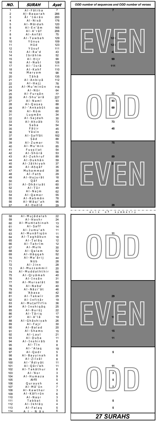
Symmetric distribution of the number of verses for surahs with odd number of verses and odd number of sequences in groups of 19 is shown in the Figure.
