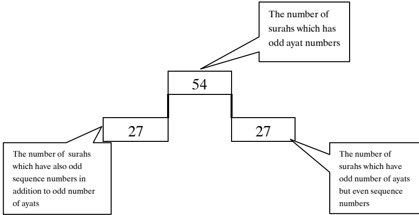
Figure-2 The equal distribution of the surahs which has odd numbered ayats is seen with respect to their sequence numbers.
