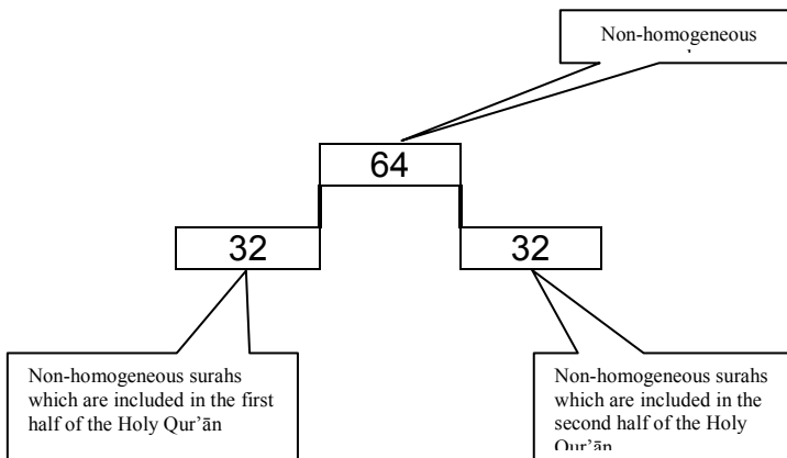
Figure-12 The equal distribution of the non-homogeneous surahs.
