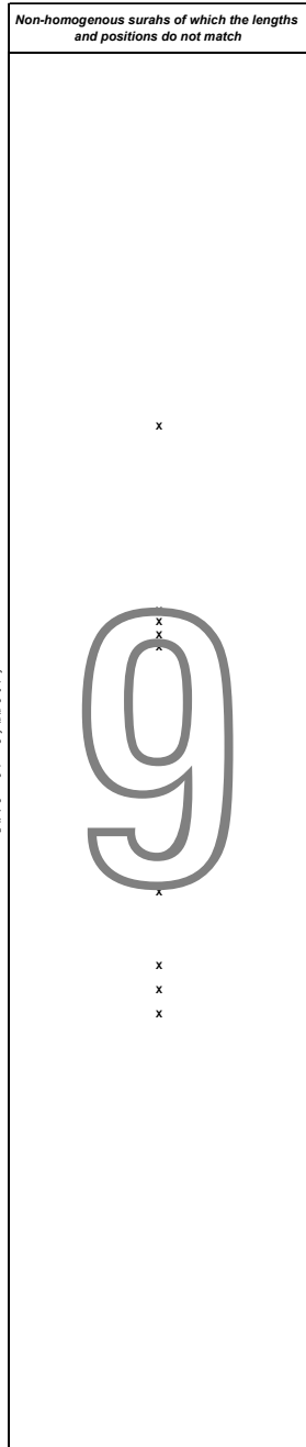
In the Figure, equal distributions of the non-homogenous surahs with not matching situation and position of the number of verses with respect to the mean, and the non-homogenous surahs with not matching lengths and positions are shown.
