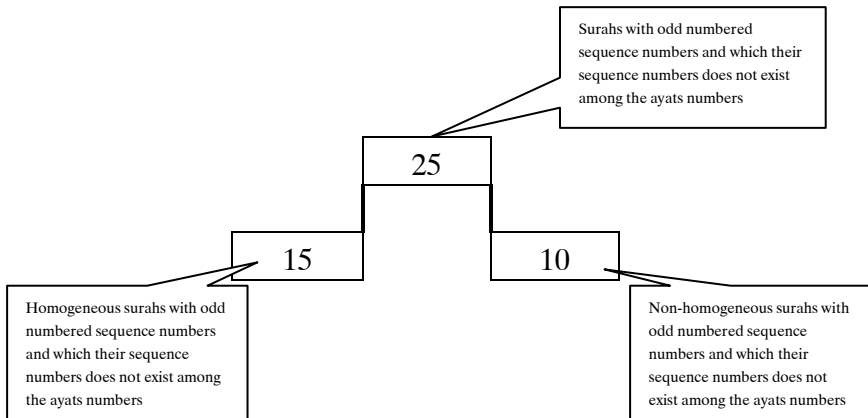
Figure-8 Distribution of the surahs with odd numbered sequence numbers and which their sequence numbers does not exist among the ayats numbers is seen.
