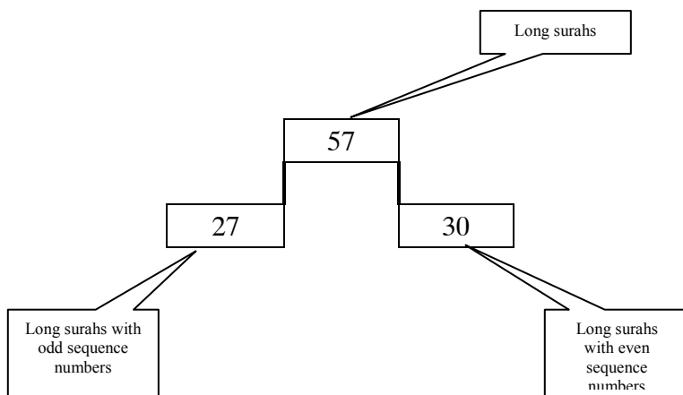
Figure-4 Distribution of the long surahs with respect to sequence number.
