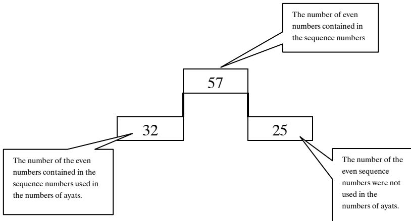
Figure-7 Distribution of the even sequence numbers which were also used in the ayat numbering and the remaining numbers is seen.
