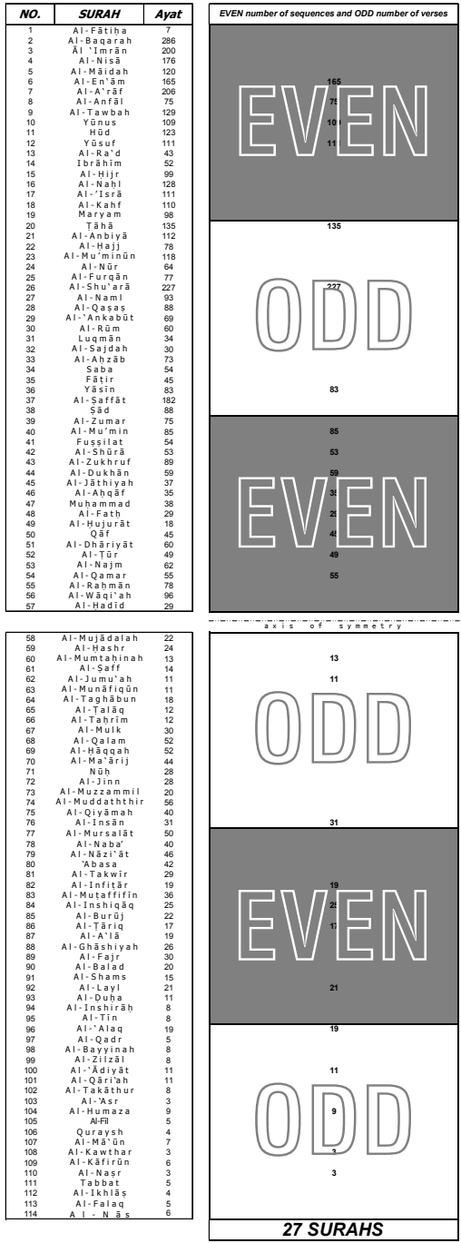
Symmetric distribution of the number of verses for surahs with even number of sequences and odd number of verses in groups of 19 is shown in the Figure.
