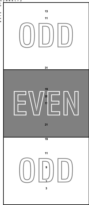
Symmetric distribution of the number of verses for the surahs with odd number of verses and the surahs with even number of verses and the surahs with even number of verses and odd number of verses in groups of 19 is shown in the Figure.
