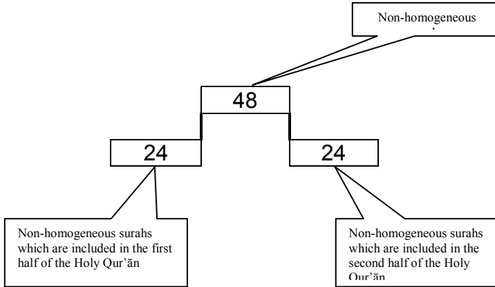
Figure-8 The equal distribution of the non-homogeneous surahs.
