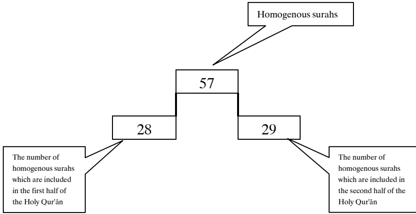
Figure-4 The distribution of the homogeneous surahs is seen.
