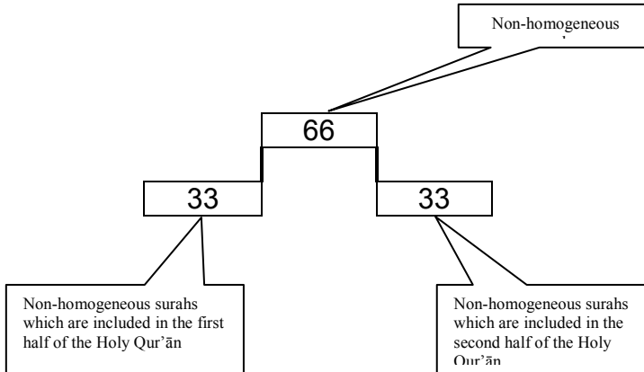
Figure-10 The equal distribution of the non-homogeneous surahs.
