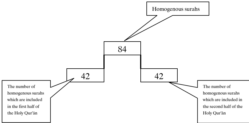
Figure-12 The equal distribution of the homogeneous surahs is seen.
