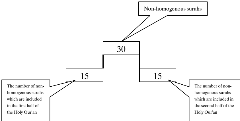
Figure-13 The equal distribution of the non-homogeneous surahs is seen.
