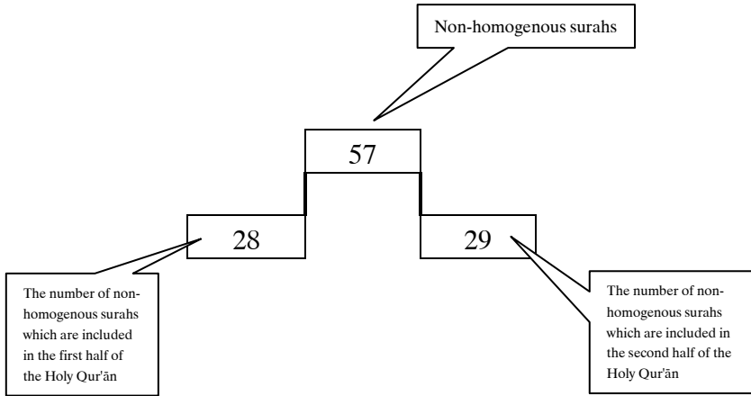
Figure-5 The distribution of the non-homogeneous surahs is seen.
