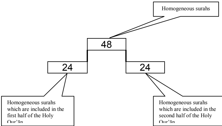
Figure-9 The equal distribution of the homogeneous surahs is seen.
