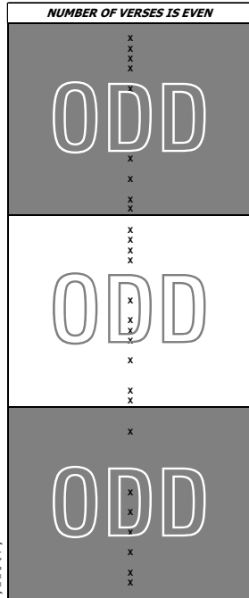
Symmetric distribution of the surahs with odd and even-number of verses in groups of 19 with respect to the number of surahs is shown in the Figure.
